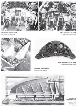
Boeing P-28 Peashooter | 131
