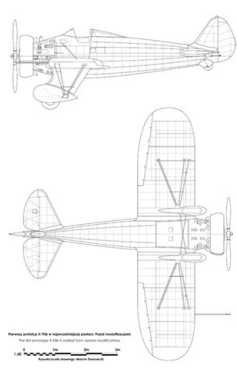
188 | Boeing P-28 Peashooter
